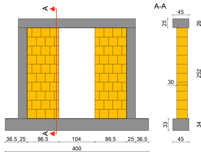
Figure 1. Test specimen
