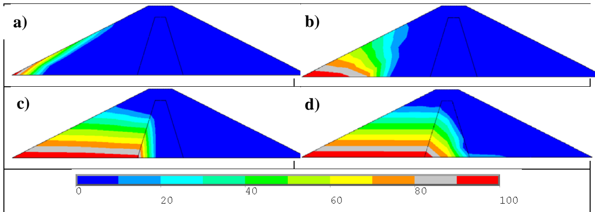
Figure 4. Pore pressure distribution inside the Dam body
