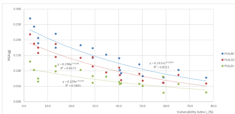
Figure 3. Vulnerability index – PGA relations ( I_v – PGA_{DL} , I_v – PGA_{SD} , and I_v – PGA_{NC} ).
